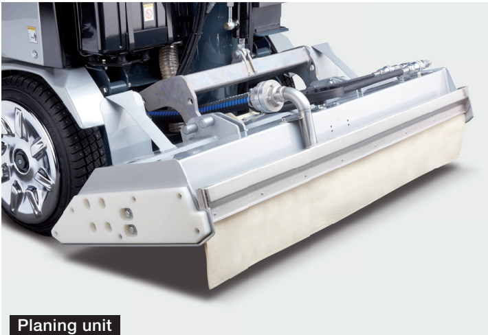
Planing unit
