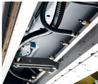
Ice wash system Multijet with suction ledge
